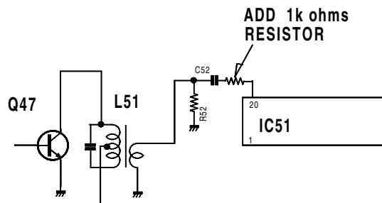
SCHEMATIC DIAGRAM
